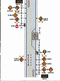
Figure 7.8. Lane Closure with TCFs - Single Lane Alternating - Short and Long Closures
